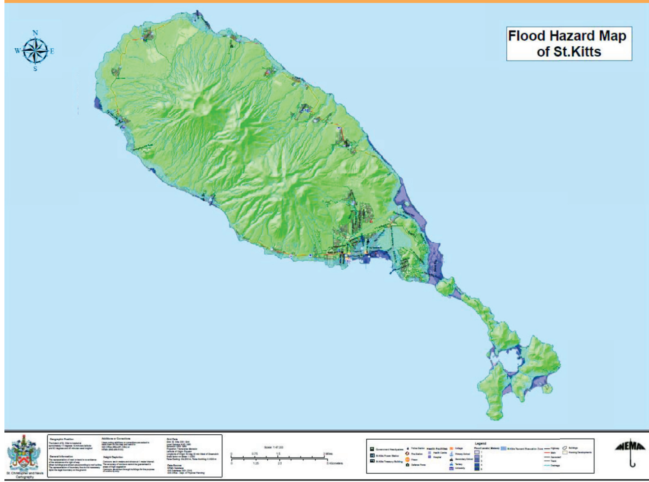
FIGURE 3.2: FLOOD HAZARD MAP OF ST. KITTS
