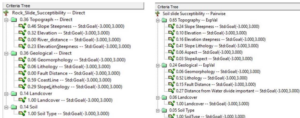
Figure 6-18: Criteria trees used for the susceptibility assessment of rockslides (left) and soil slides (right)
