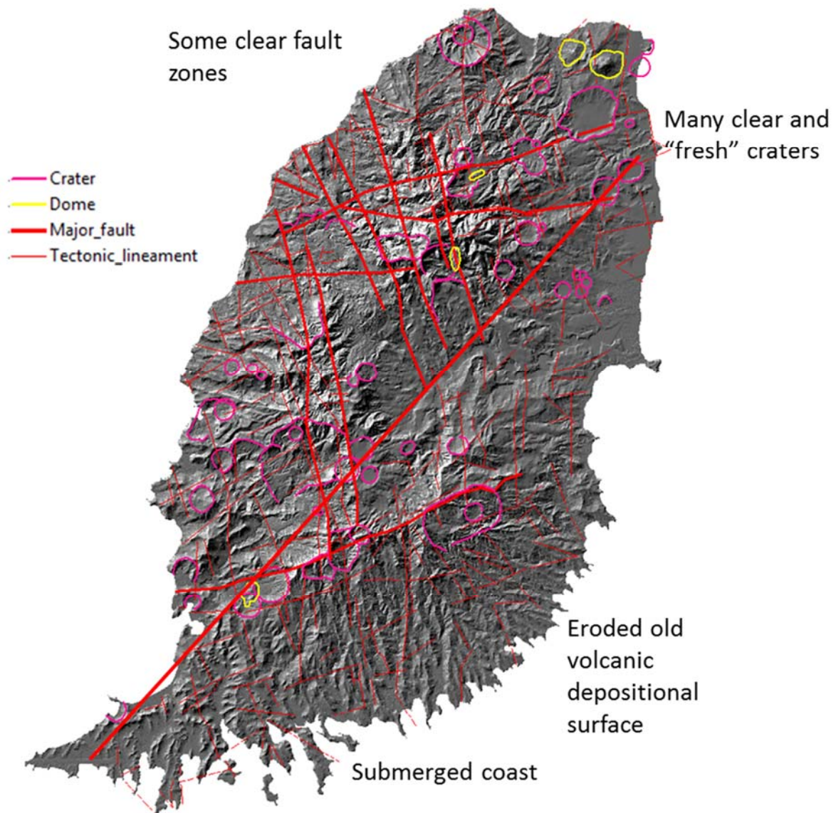
Figure 5-5. Geomorphological interpretation of Grenada (Van Westen) outlining the visible craters, domes, major faults and lineaments.
