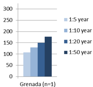
Figure 3-3. Maximum daily rainfall (mm) at Maurice Bishop international airport for return periods of 5, 10, 20 and 50 years.
