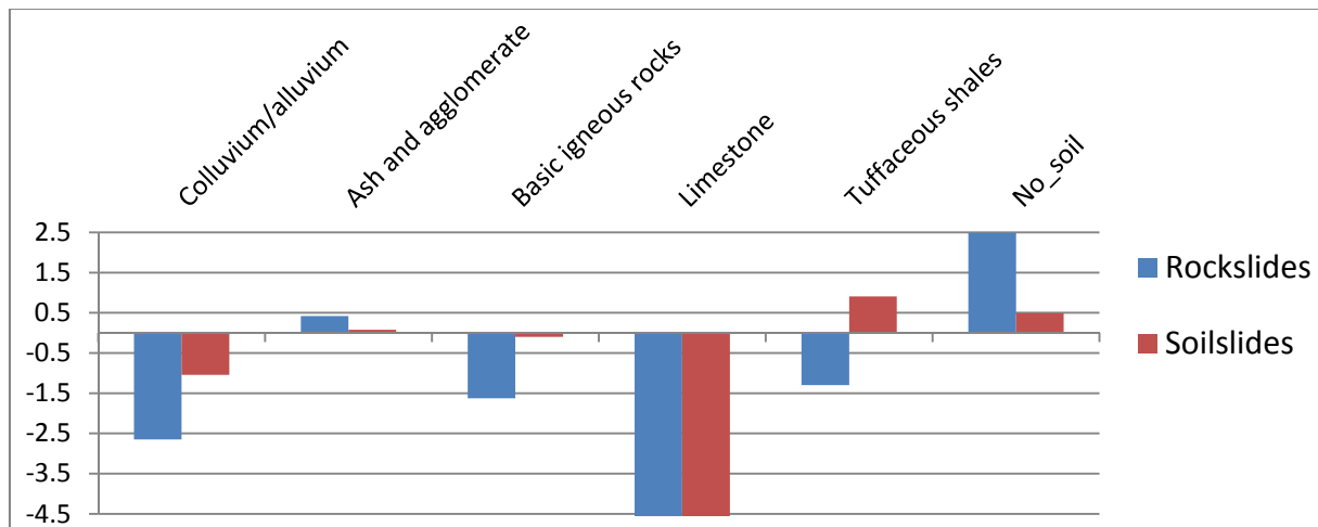
Figure 6-14: Contrast factors for parent materials of soils for rockslides and soil slides.
