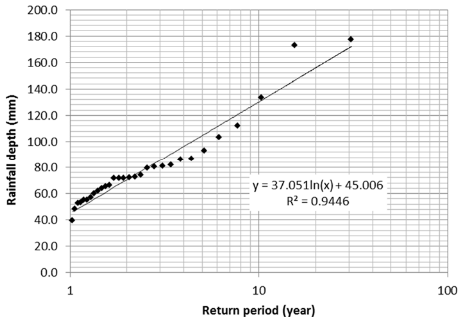
Figure 3-2. Frequency magnitude of annual maximum daily rainfall at Maurice Bishop international airport (1986-2014).
