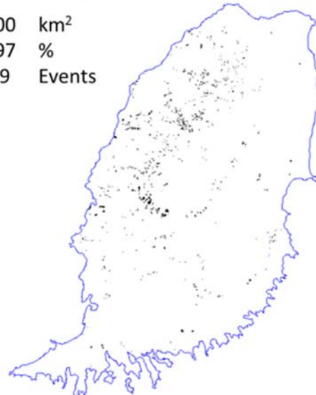
Figure 6-4: Landslide inventory maps for rockslides and soil-related landslides that were used in the analysis.
