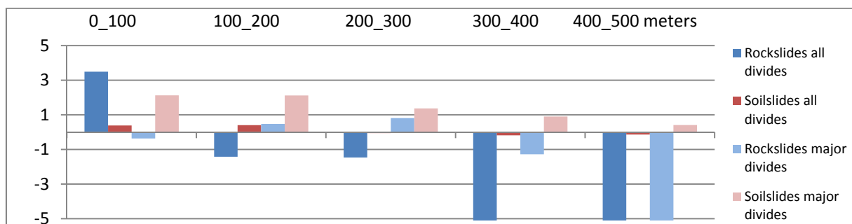
Figure 6-11: Contrast factors for distance to ridges for rockslides and soilslides.
