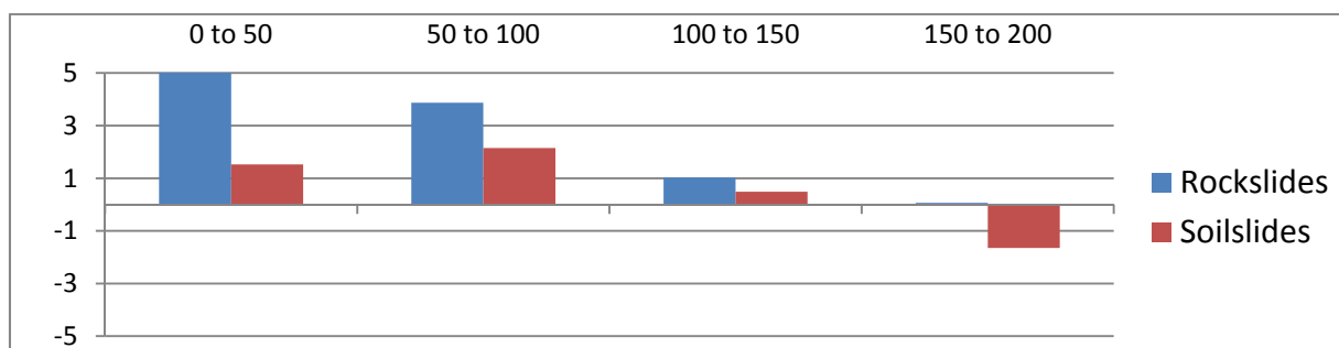
Figure 6-10: Contrast factors for distance to the coast for rockslides and soil slides.
