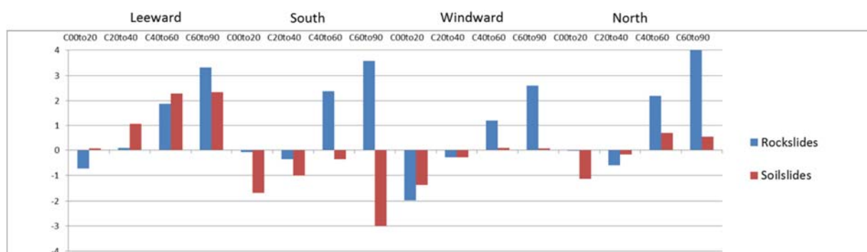
Figure 6-8: Contrast factors for the combination of the main exposure classes and slope steepness classes for rockslides and soil slides.
