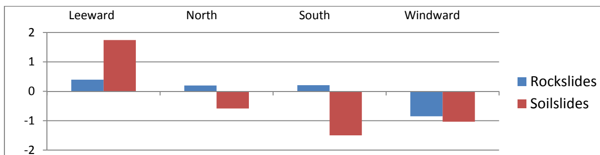
Figure 6-7: Contrast factors for main exposure classes for rockslides and soil slides.
