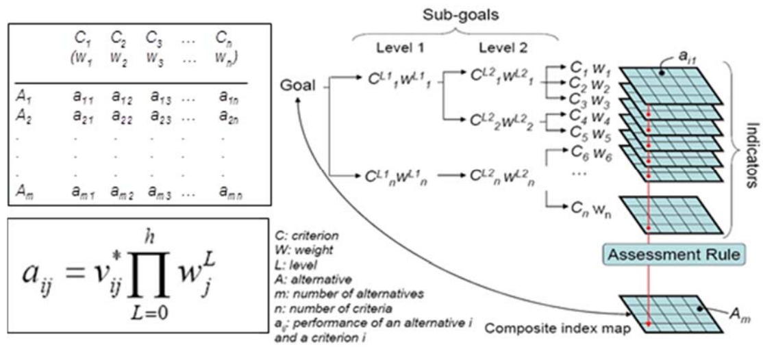
Figure 6-17: Schematic procedure for spatial multi-criteria evaluation based on the analytical hierarchical process
