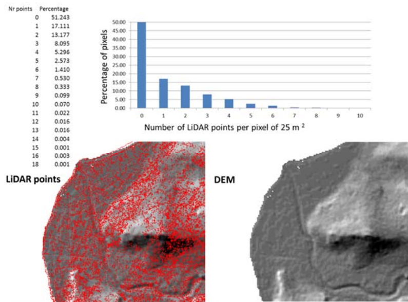
Figure 5-1: The Digital Elevation Model for Grenada was generated from LiDAR points. The table and graph show the number of points per pixel of 25 m 2 (5 by 5 meter pixel). The map on the lower left shows the LiDAR points for a sample area around Gouyave, and the image on the lower right the resulting DEM.
