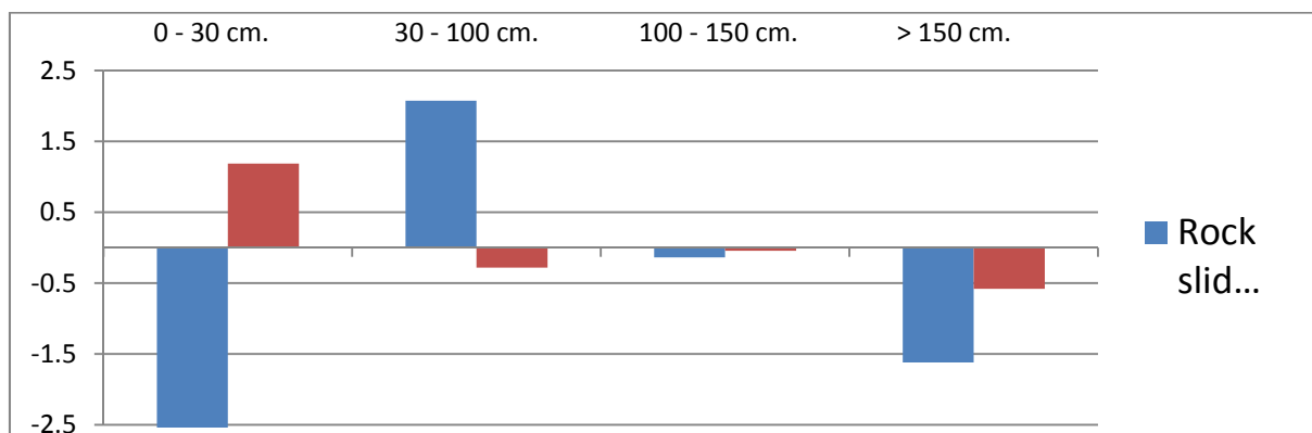
Figure 6-15: Contrast factors for soil depth classes for rockslides and soil slides.
