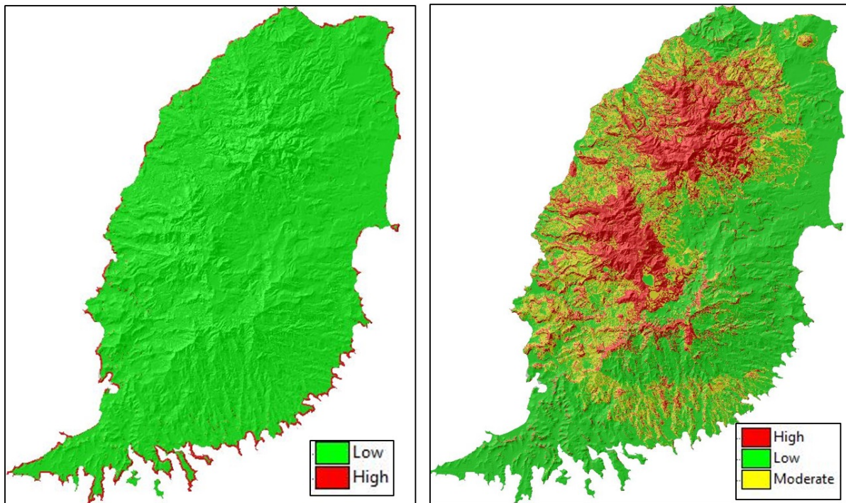
Figure 6-20: Classified landslide susceptibility maps for rockslides (left) and soil slides (right)
