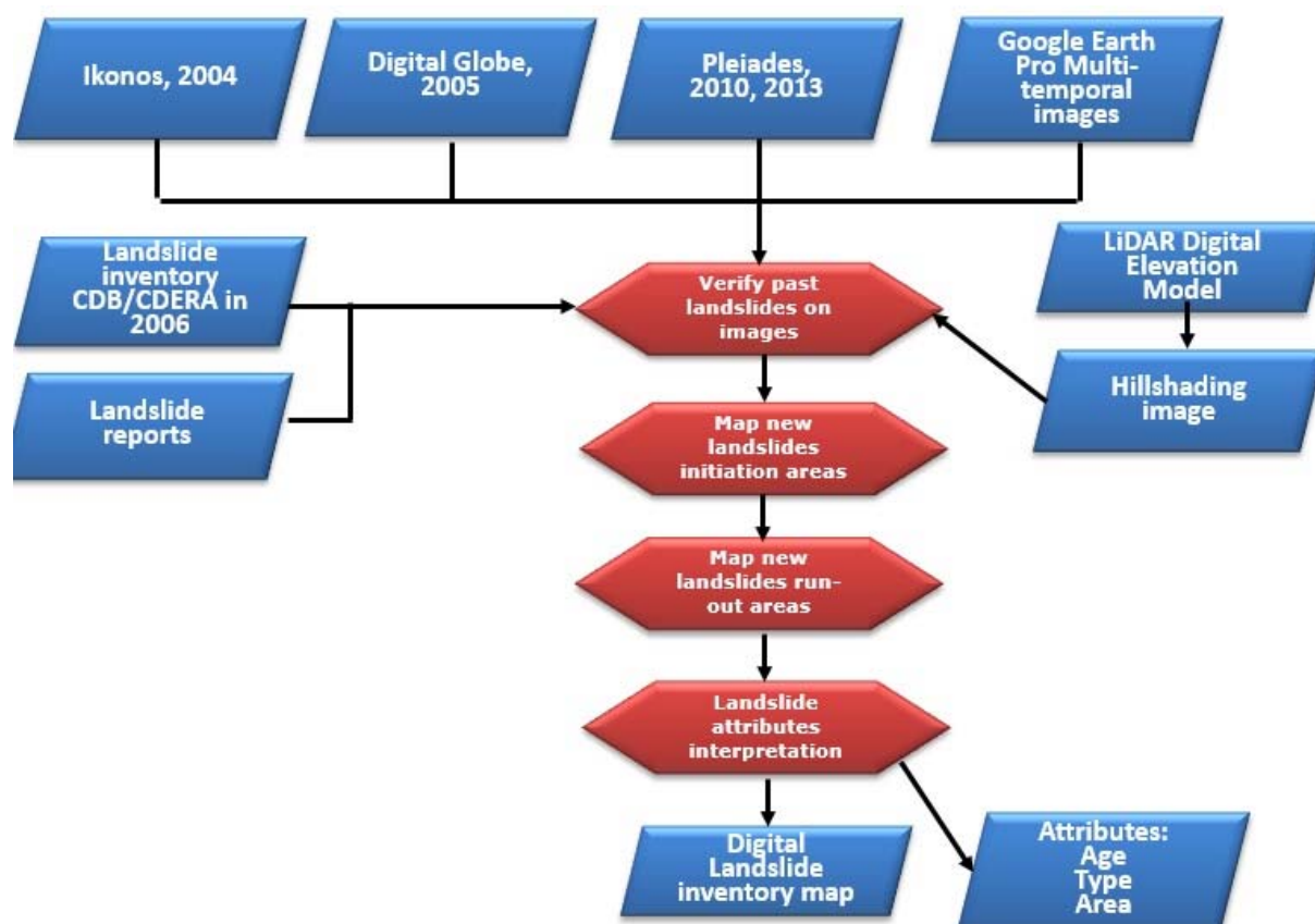
Figure 4-2: Method used for the generation of a landslide inventory map for Grenada
