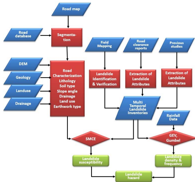
Figure 8-2: Method used for assessing the landslide susceptibility along the national road network in Grenada.
