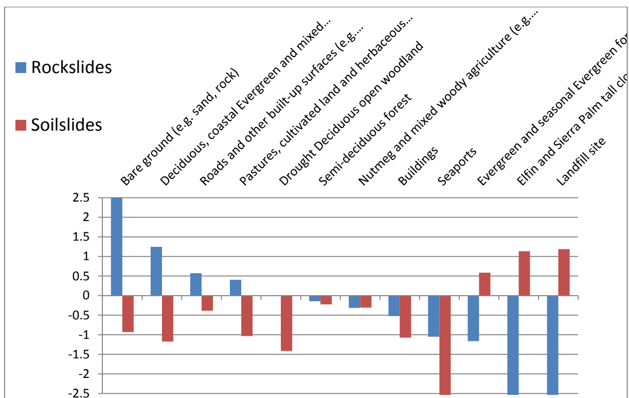
Figure 6-16: Contrast factors for land use classes for rockslides and soil slides.
