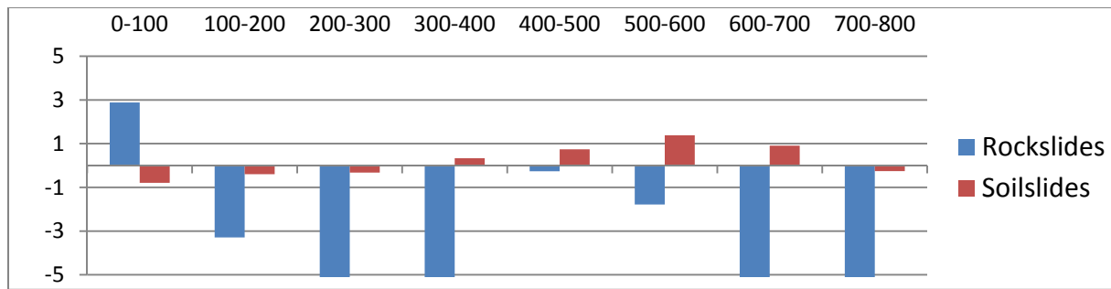
Figure 6-9: Contrast factors for elevation classes for rockslides and soil slides.
