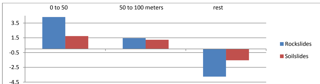
Figure 6-13: Contrast factors for distance to roads for rockslides and soilslides.
